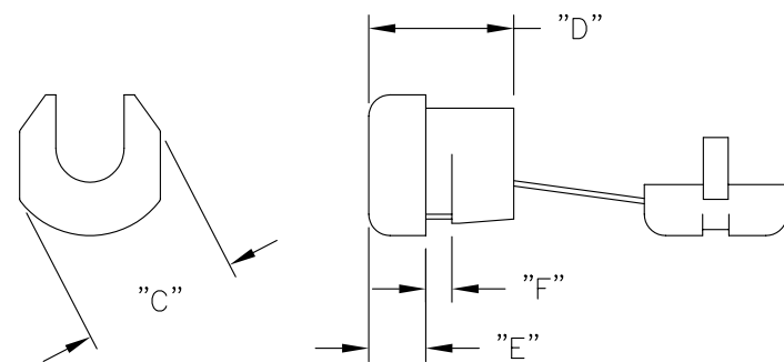
BUSHING DIMENSIONS
